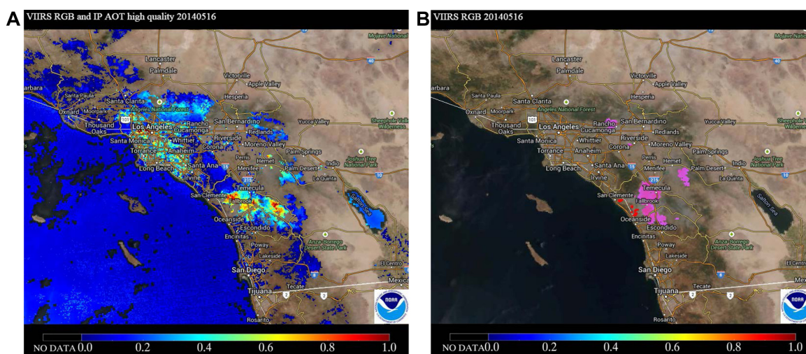
Figure 8. (A) The left panel shows VIIRS 750-m \times 750-m resolution Intermediate Product (IP) aerosol optical depth (AOD) NRT imagery from the IDEA web site for Southern California on May 16, 2014. Areas of high AOD, shown by the red, orange, and yellow colors, north of San Diego, near Temecula, Oceanside, and Fallbrook correspond to smoke from the wildfires burning in northern San Diego County. Areas of high AOD over Los Angeles are due to urban haze. (B) The right panel shows VIIRS true color (RGB) NRT imagery from the IDEA web site for Southern California on May 16, 2014. Fire hotspots identified by VIIRS are overlaid as small red dots. The pink shaded areas correspond to the VIIRS smoke mask. Smoke from the San Diego County wildfires is evident as a light gray feature in the RGB image, but it is difficult to discern. The pink VIIRS smoke dust mask captures the thickest parts of the smoke plume, aiding in identification and tracking.
